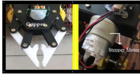
Fig. 3 Wrist and end effectors with Stepper Motor
