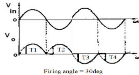
Fig (6) Output voltage waveform for firing angle = 30^\circ deg
