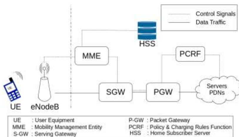
Fig. 1 LTE Architecture
