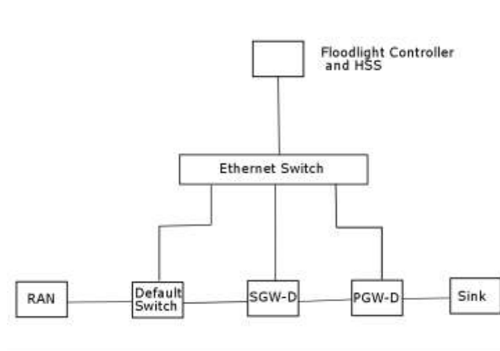
Fig. 5 Experimental Setup
