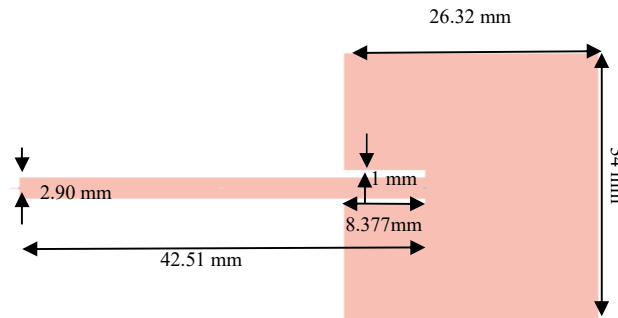
Figure 2: Designed microstrip patch antenna
