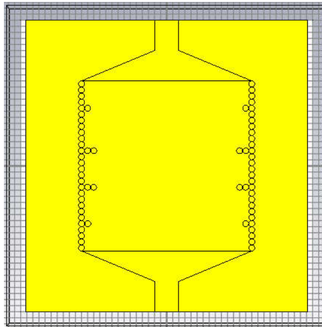
Fig.4.Proposed SIW Filter Design structure and its parameters.
